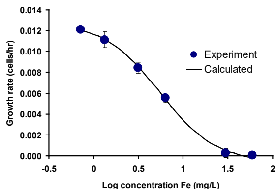
Fig. 1. The effect of Nanofer 25S on the growth rate for I. galbana .
