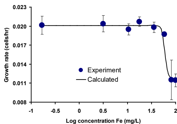
Fig. 3. The effect of Fe^{3+} on the growth rate for I. galbana .
