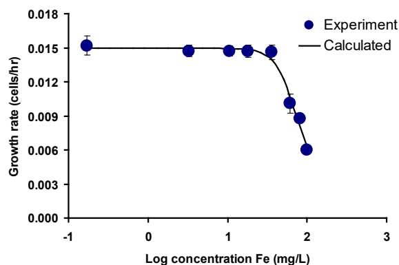
Fig. 2. The effect of Nanofer STAR on the growth rate for I. galbana .
