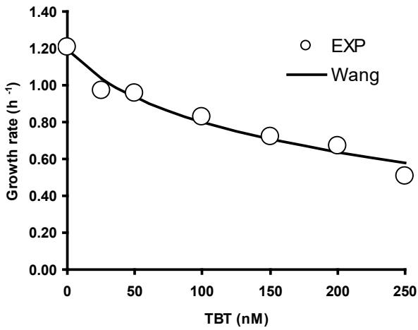
Fig. 1. The effect of increasing concentrations of TBT to the specific growth rate of B. subtilis as fitted to the Wang model.
