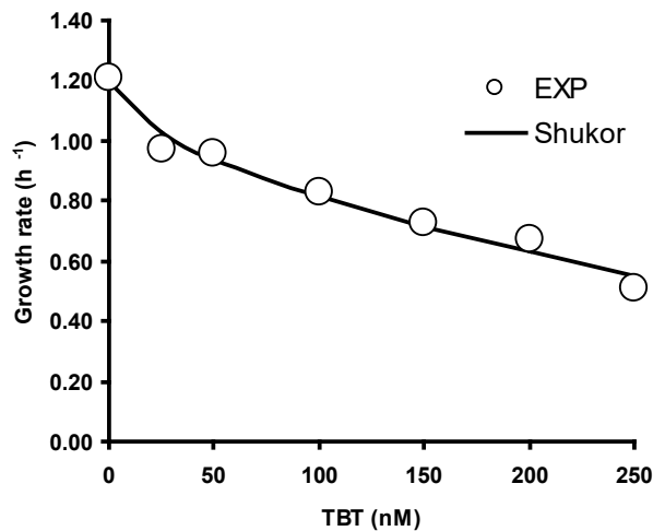
Fig. 5. The effect of increasing concentrations of TBT to the specific growth rate of B. subtilis as fitted to the Shukor model.
