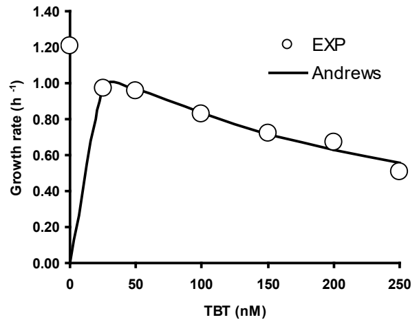
Fig. 4. The effect of increasing concentrations of TBT to the specific growth rate of B. subtilis as fitted to the Andrew model.
