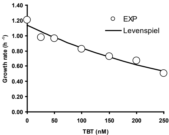
Fig. 2. The effect of increasing concentrations of TBT to the specific growth rate of B. subtilis as fitted to the Han-Levenspiel model.
