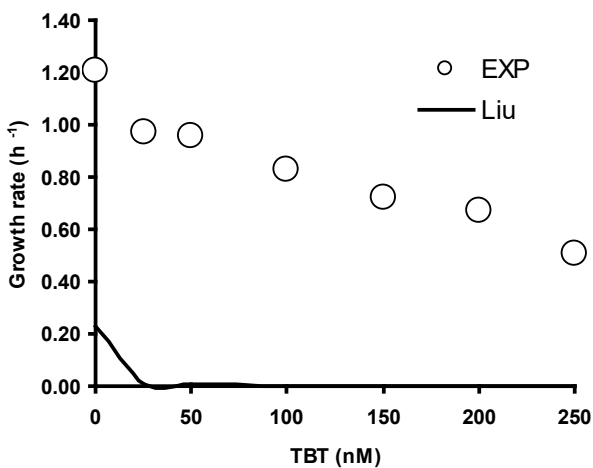
Fig. 2. The effect of increasing concentrations of TBT to the specific growth rate of B. subtilis as fitted to the Liu model.
