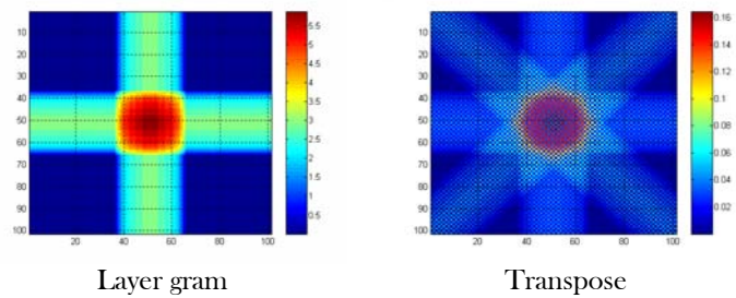
Figure 4 Simulated images for a 400 \mu\text{m} sample
