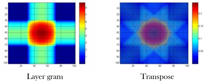
Figure 3 Simulated images for a 600 \mu\text{m} sample
