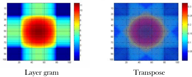
Figure 2 Simulated images for a 800 \mu\text{m} sample
