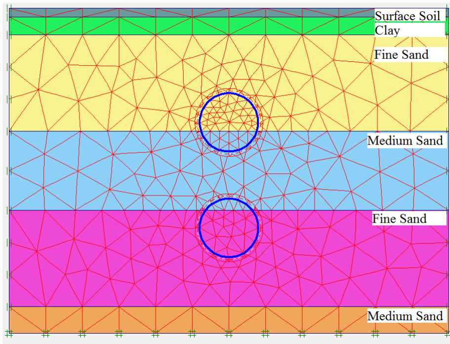
Figure 4 : FEM mesh in simulations of the typical cross-section of the Metro No. 1 using PLAXIS 2D v8.5 software.
