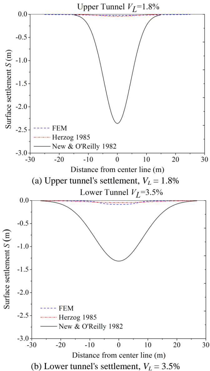
Figure 5: Surface settlement analysis for the study cross-section
