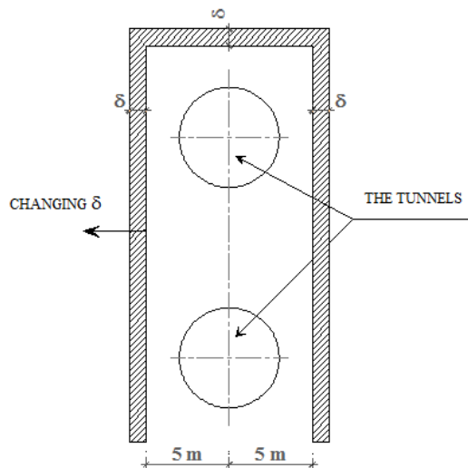
Figure 6 : The sub-soil reinforced by Jet Grouting at the cross-section at the Opera House (URMB 2010)
