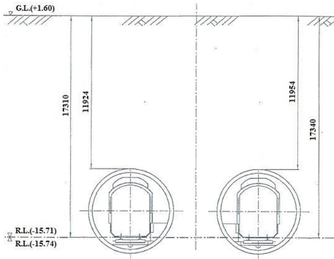
(a) 2-parallel tunnel cross-section
