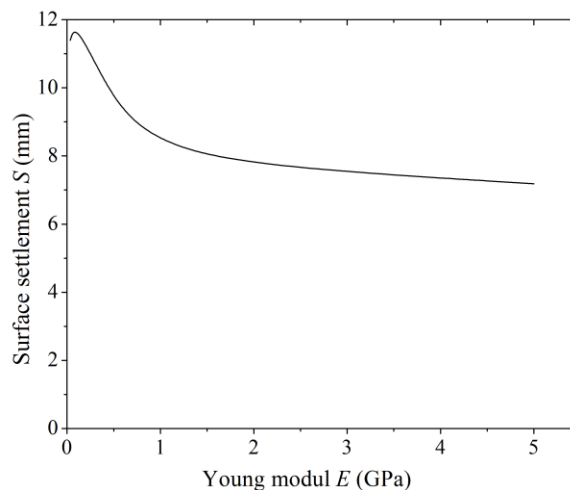
Figure 7 : Relationship of surface settlement and E at \delta = 1 m
