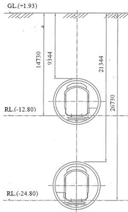
(b) 2-vertical tunnel cross-section
