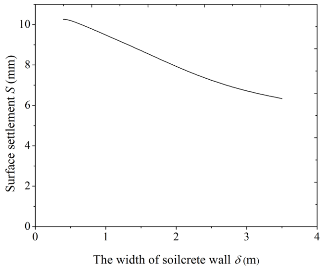
Figure 8 : Relationship of surface settlement and \delta at E = 500 MPa
