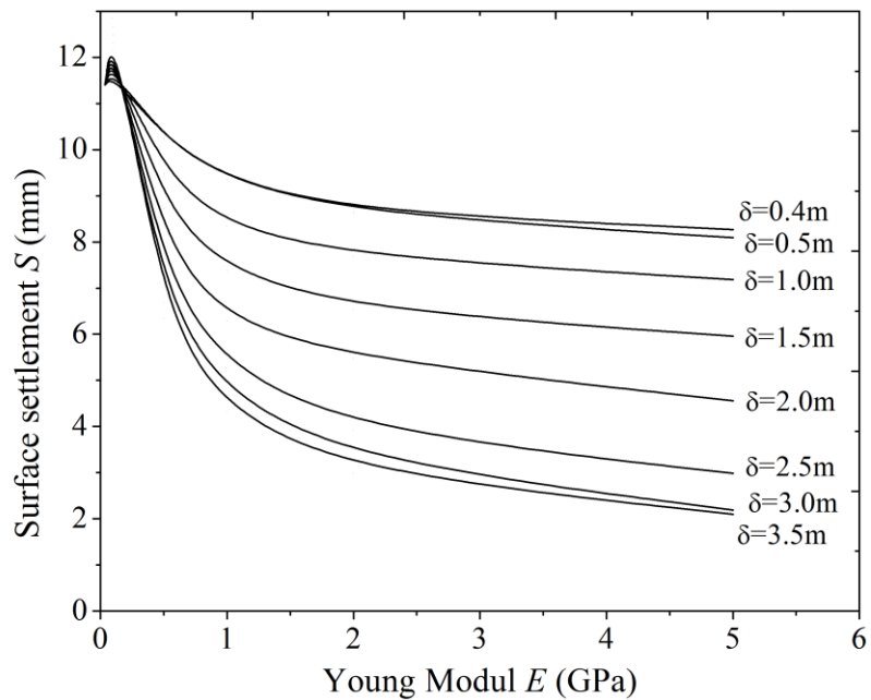
Figure 9 : Relationship of surface settlement and the characteristics of soilcrete ( E & \delta )
