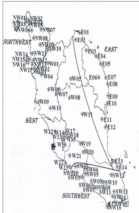
Figure 1 The locations of the rain gauges stations over Peninsular Malaysia
