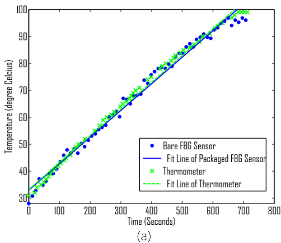
Figure 5 Temperature characteristics curve of bare and packaged sensor
