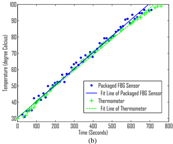
Figure 6 Temperature measurement of (a) bare FBG sensor, and (b) packaged sensor
