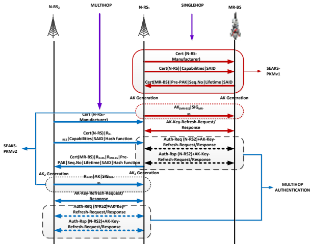
Fig 2 SEAKS authentication protocol
