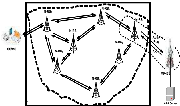
Fig.4 Authentication of N-RS 1 with MR-BS
