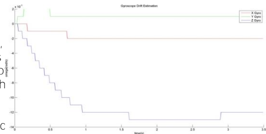
Figure 15 Convergence of gyroscope drift estimation
