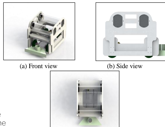
Figure 3 Solidworks rendered images of ROV
