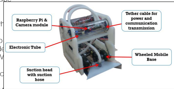
Figure 7 Actual design of ROV developed
