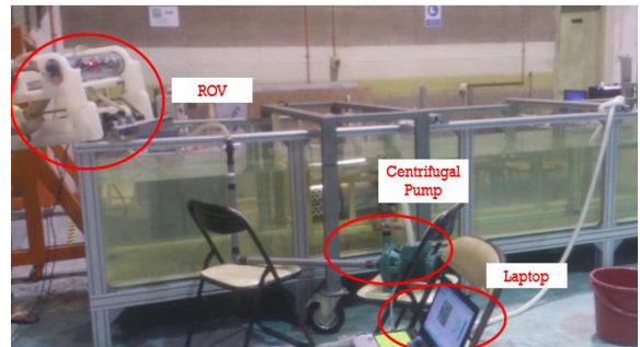
Figure 20 ROV underwater testing set-up
