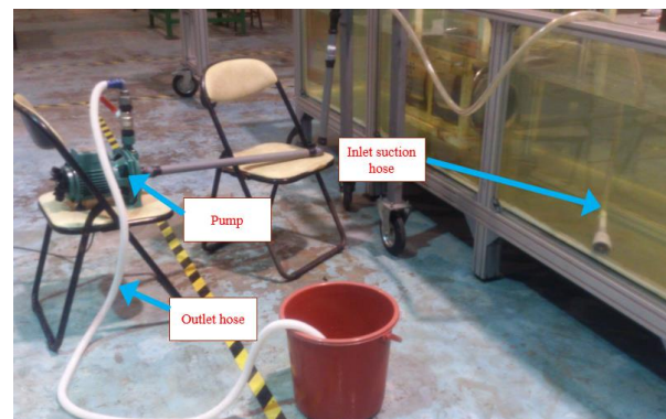
Figure 11 Cleaning set-up
