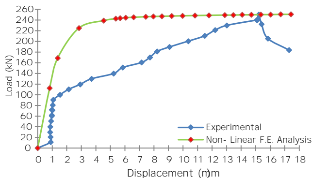
Figure 6 Experimental and simulated results for SRLWAC beam
