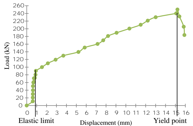
Figure 5 Load versus mid-span displacement of SRLWAC beam
