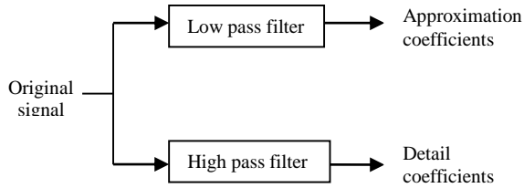
Figure 2 Stationary Wavelet Transform decomposition
