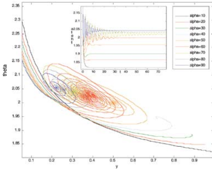
Fig. 15: Phase-plane of model equations at K_c = 10 and D = 50 at various \alpha
