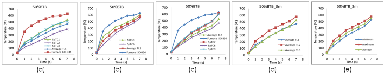
Figure 6 Evaluation of mean temperature along the column for 50.0 % degree of utilisation
