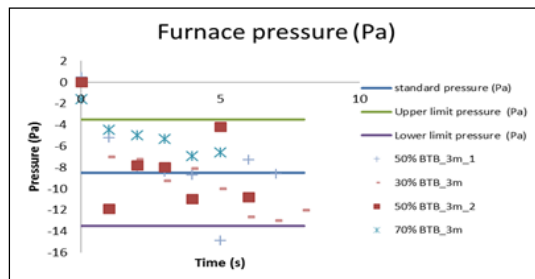
Figure 3 Furnace pressure inside furnace
