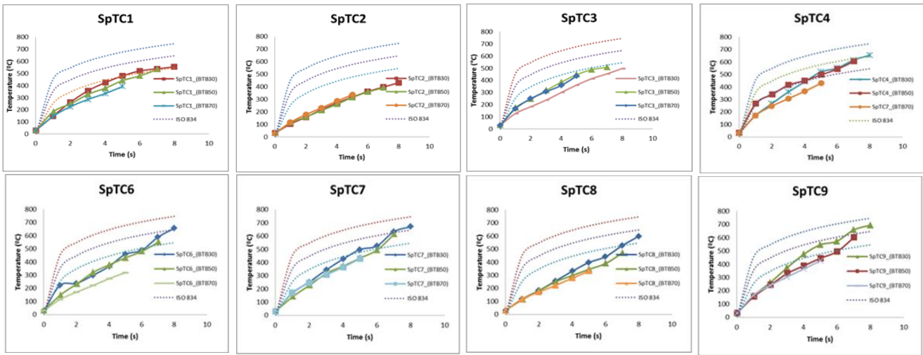
Figure 4 Temperature rise in built-up back to back column
