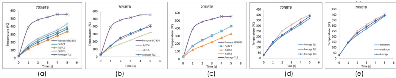
Figure 7 Evaluation of mean temperature along the column for 70.0 % degree of utilisation
