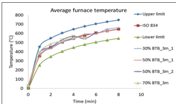
Figure 2 Average furnace temperature
