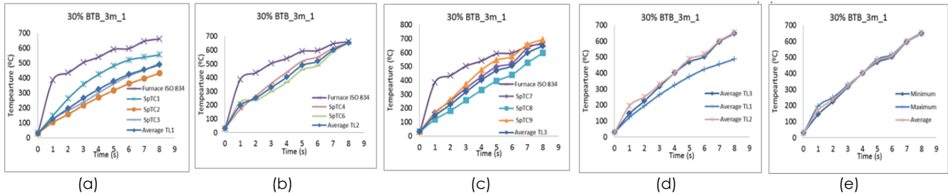
Figure 5 Evaluation of mean temperature along the column for 30.0 % degree of utilisation
