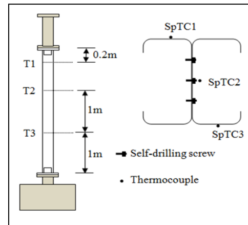
Figure 1 Location of thermocouple on the column
