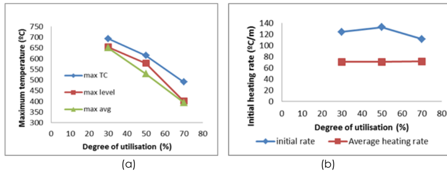
Figure 8 (a) Evaluation of critical temperature (b) Heating rate of the column
