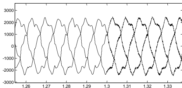
Figure 9 Nonlinear current being compensated with the passive components and the active component
