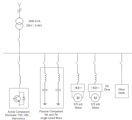
Figure 7 HPAPF with active and passive components installed
