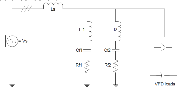
Figure1 Single tuned passive filter diagram
