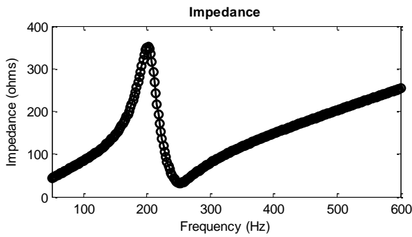
Figure 2 Branch Impedance versus Frequency diagram of a typical single tuned passive filter
