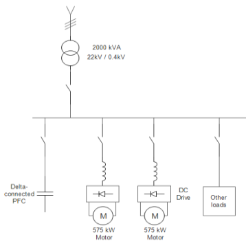
Figure 5 Basic electrical diagram of the cable car transport system using DC drives in Danang, Vietnam
