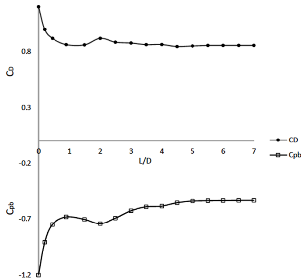
Figure 2. Variation of C_{pb} and C_D with downstream plate's length ratio. L/D \leq 2 (Apelt et al., 1973), 2 \leq L/D \leq 7 (Apelt & West, 1975).
