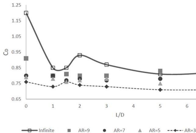
Figure 7. Mean C_D in different downstream plate's length ratio. Infinite cylinder (Apelt & West, 1975), Finite cylinder (Igbalajobi et al., 2013).
