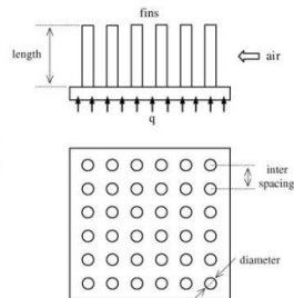
Fig.3. Cylindrical structure cooling fin
