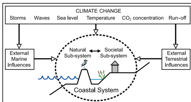
Figure 1 Schematic framework representing major climate change factors, including external marine and terrestrial influences [16]
