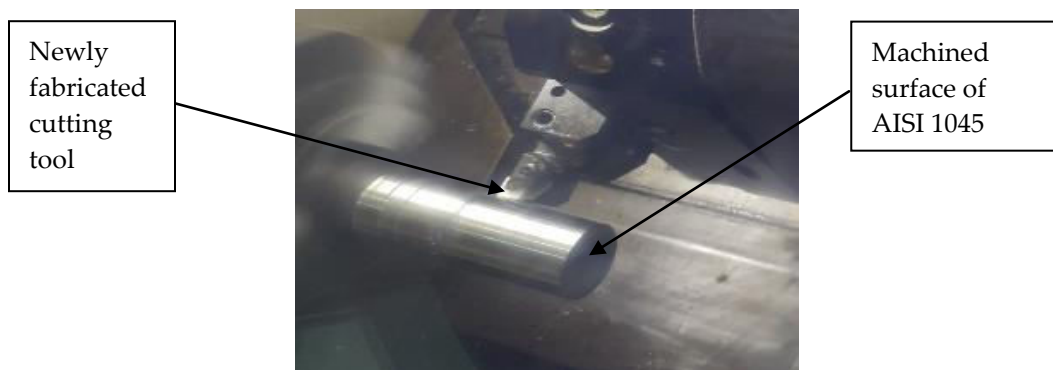
Figure 4: Alumina cutting tool on tool holder when machining AISI 1045
