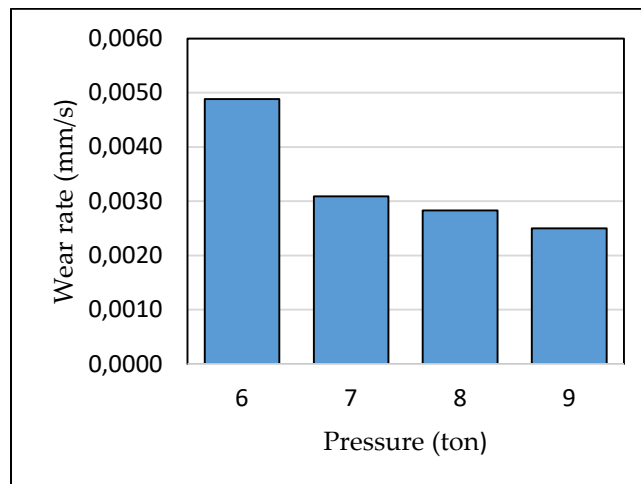
Figure 6: Effect of hydraulic pressure (tons) on wear rate (mm/s)
