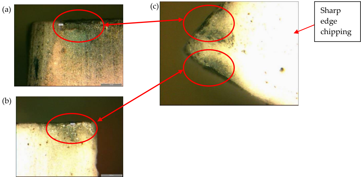
Figure 7: Wear at the edge of cutting tools: (a) right flank side of tool, (b) left flank side of tool and (c) top side of tool
