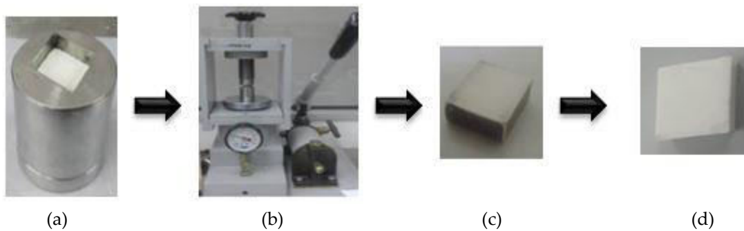
Figure 3: The compaction method procedures: (a) Powder pours into the mould, (b) The mould is pressed by hydraulic hand press, (c) The body is ejected out from the mould and (d) Ceramic cutting tool after sintering the white body colour
