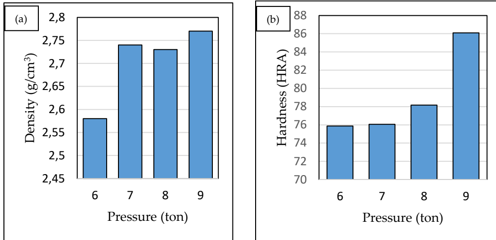
Figure 5: (a) Effect of hydraulic pressure (tons) on density (g/cm 3 ) and (b) Effect of hydraulic pressure (tons) on hardness (HRA)
