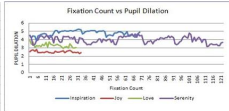
Figure 24: Fixation Count vs Pupil Duration for Subject 10
