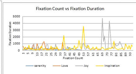
Figure 6: Fixation Count vs Fixation Duration for Subject 2
