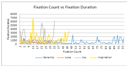
Figure 13: Fixation Count vs Fixation Duration for Subject 9
