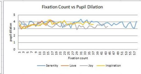
Figure 20: Fixation Count vs Pupil Duration for Subject 6
