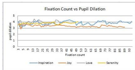
Figure 16: Fixation Count vs Pupil Duration for Subject 2
