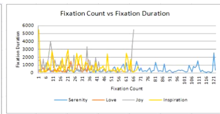
Figure 8: Fixation Count vs Fixation Duration for Subject 4
