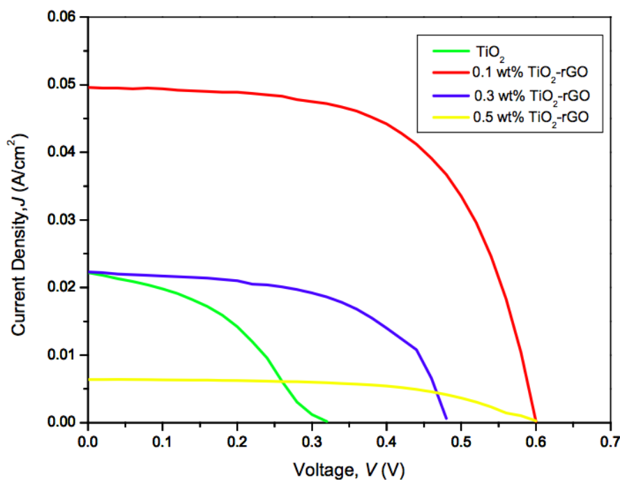
Figure 4. J-V curve of DSSC
